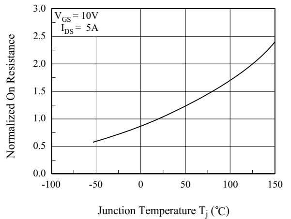
R_{DS(ON)} - T_j
